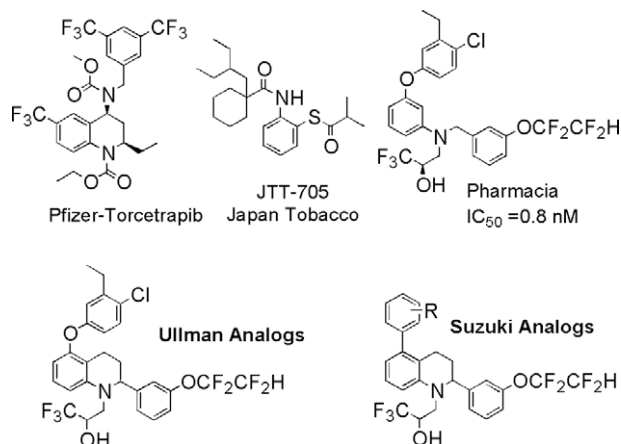
Figure 1. Structures of current CETP inhibitors.
