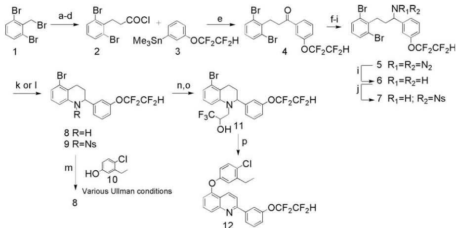
Scheme 1. Reagents and conditions: (a) (\text{EtO}_2\text{C})_2\text{CHNa} , DMF, 50 °C, 75%; (b) NaCl, DMSO, water, 180 °C, quantitative; (c) 3 N NaOH, THF, reflux, quantitative; (d) oxalyl chloride, DCM, quantitative; (e) \text{Pd}_2\text{DBA}_3 , DIEA, THF, 50 °C, 66%; (f) \text{NaBH}_4 , MeOH, 84–94%; (g) \text{MsCl} , TEA, DCM, quantitative; (h) \text{NaN}_3 , DMF, 50 °C, 92–97%; (i) \text{Me}_2\text{S}\cdot\text{BHCl}_2 , DCE, reflux, then HCl, 95%; (j) \text{NsCl} , TEA, DCM, 85%; (k) 10% \text{CuI} , \text{K}_3\text{PO}_4 , 40% o\text{-(OH)C}_6\text{H}_4\text{CONEt}_2 , ~25%; (l) \text{CuI} , \text{Cs}_2\text{CO}_3 , DMSO, 90 °C, 90%; (m) Ullman conditions (n) \text{HSCH}_2\text{CO}_2\text{H} , LiOH, DMF, 88%; (o) \text{Yb}(\text{OTf})_3 , 1,1,1-trifluoroethoxypropane; DCE, 50 °C; (p) \text{CuCl} , \text{Cs}_2\text{CO}_3 , (\text{CH}_3)_3\text{CCOCH}_2\text{COC}(\text{CH}_3)_3 , phenol 9 , NMP, 120 °C.
